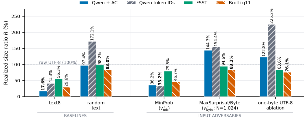
Figure 1: End-to-end compression across natural vs. adversarial inputs. Realized size ratio R for Qwen+AC, fixed-width Qwen token-ID, FSST [12], and Brotli. Bold values mark the smallest stream for each input. All streams are round-trip-verified. Qwen model weights, tokenizer table are excluded.
